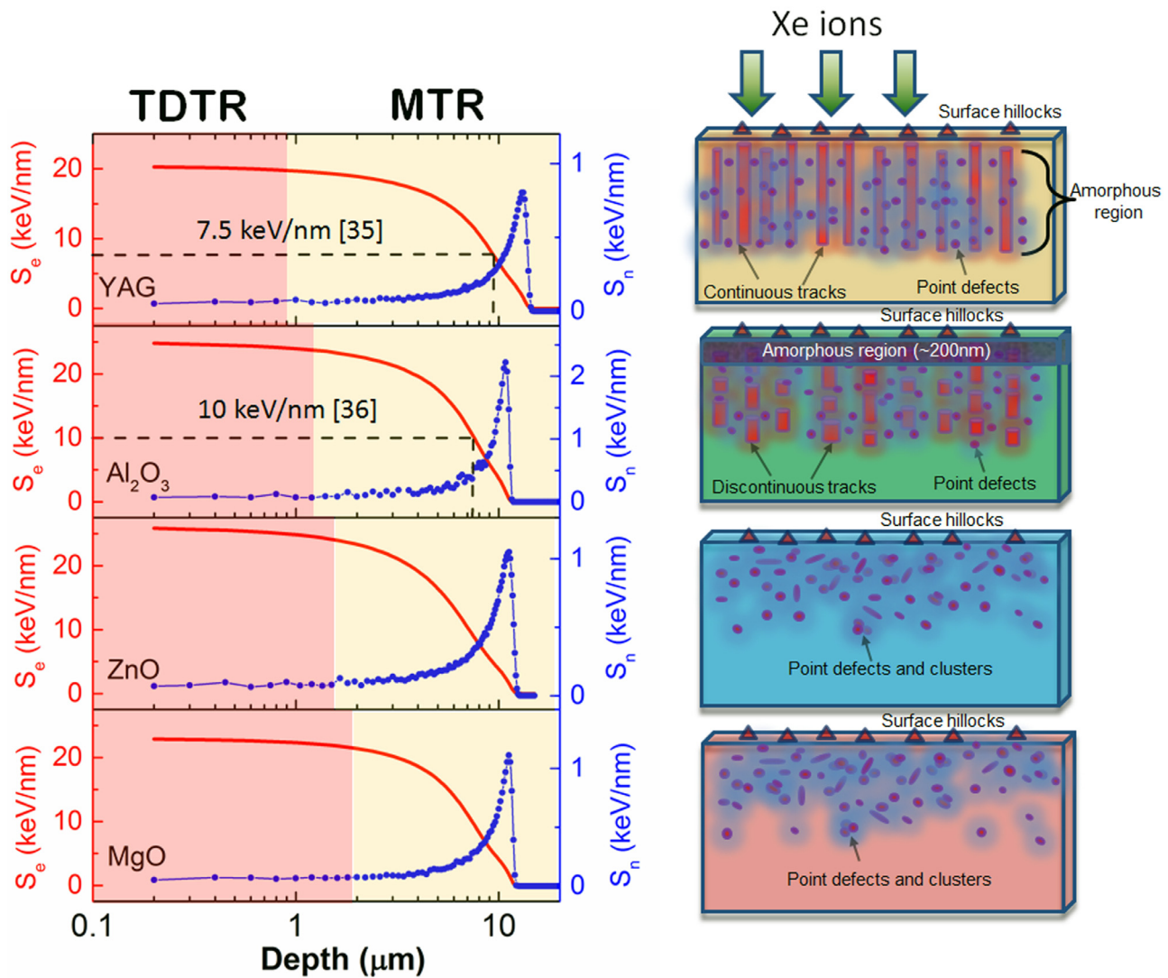
Fig. 1. Left hand side image shows TRIM calculation of 167 MeV Xe irradiated oxides. S_e and S_n indicate electronic and nuclear energy loss, respectively. The graph also shows that TDTR heat penetration is sensitive only up to \sim 2 \mu\text{m} depth, while MTR covers up to 20 \mu\text{m} . Dashed lines correspond to maximum depth where ion tracks are visible in SHI irradiated YAG [35] and \text{Al}_2\text{O}_3 [36]. The right hand side shows irradiation direction and schematic diagrams of the respective irradiated oxides indicating different types of defects induced by SHIs.
