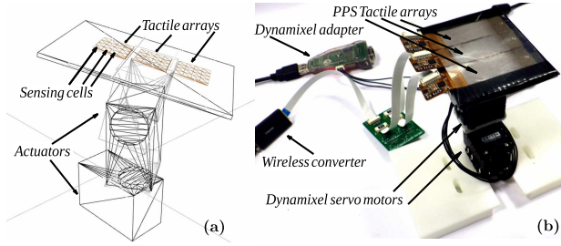
Fig. 10: (a) Experimental platform with 3 \times 6 \times 4 DigiTacts Pressure Profile System tactile sensing arrays for validation of a continuously changing tactile image. (b) The real 2dof platform.
