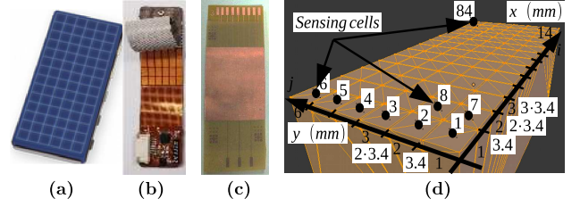
Fig. 2: Tactile sensing arrays: (a) WeissRobotics, (b) PressureProfileSystems, (c) Tactile sensing array developed by Laboratory for Integration of Systems and Technology of the French Alternative Energies and the Atomic Energy Commission, (d) 3D mesh model of the 6 \times 14 WeissRobotics tactile sensing array.
