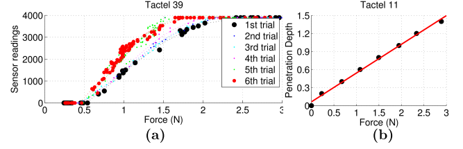
Fig. 6: (a) Step responses of the same tactel from multiple trials (tactel 39 in this case study). (b) Maximum penetration depth and ground-truth force measurements.
