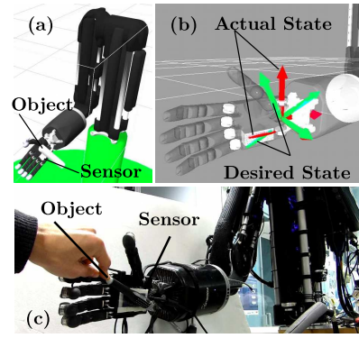
Fig. 12: Edge orientation servoing in the Cartesian space.
