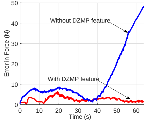
Figure 12: The comparison of the error convergence of the force during the bent (in two planes) bar exploration without (baseline approach [7] in blue) and with (proposed approach in red) use of the control of the DZMP feature. The desired values were set to 5 N.
