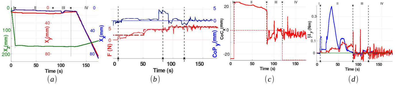
Figure 10: Plots of the evolutions of: (a) the position of the end-effector along x- (red), y- (blue), and z- (green) axes, (b) feedback (solid line) and desired (dashed line) forces (red), and feedback (solid) and desired (dashed) CoP_y (blue), (c) the feedback (solid) and desired (dashed line) CoP_x , (d) the feedback DZMP_y (red) and its desired value (green) compared with ground-truth moment of force (blue).
