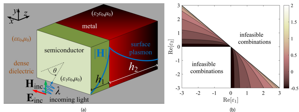
Figure 1. (a) A simple bilayer comprising a semiconducting slab of thickness h_1 and relative permittivity \varepsilon_1 as well as a metallic layer of thickness h_2 and relative permittivity \varepsilon_2 . The structure is placed into a dense dielectric of relative permittivity \varepsilon and gets obliquely illuminated by a plane wave of light with wavelength \lambda that propagates along a direction making angle \theta with the normal direction. The setup is designed to host surface plasmon resonances regarding the magnetic field magnitude |\mathbf{H}(z)| along the interface between the two media ( z = 0 ). (b) The variation of the decimal logarithm of the normalized propagation constant \log(\beta/k_0) across the map of the two permittivities (\varepsilon_1, \varepsilon_2) of the used media. Lossless designs are considered ( \text{Im}[\varepsilon_1] = \text{Im}[\varepsilon_2] = 0 ).
