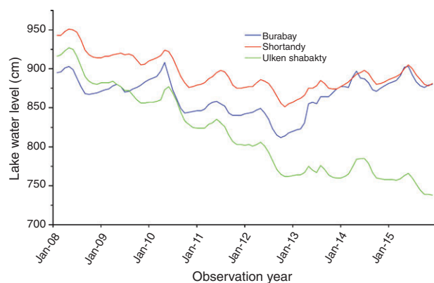
FIGURE 5 | Lake water levels 2008–2015: Shortandy Lake (brown), Burabay Lake (blue), Ulken Shabakty (green). 16 Zero datum level (msl, Baltic reference): Shortandy Lake—380.04 m; Burabay Lake—311.23 m; Ulken Shabakty—289.5 m.
