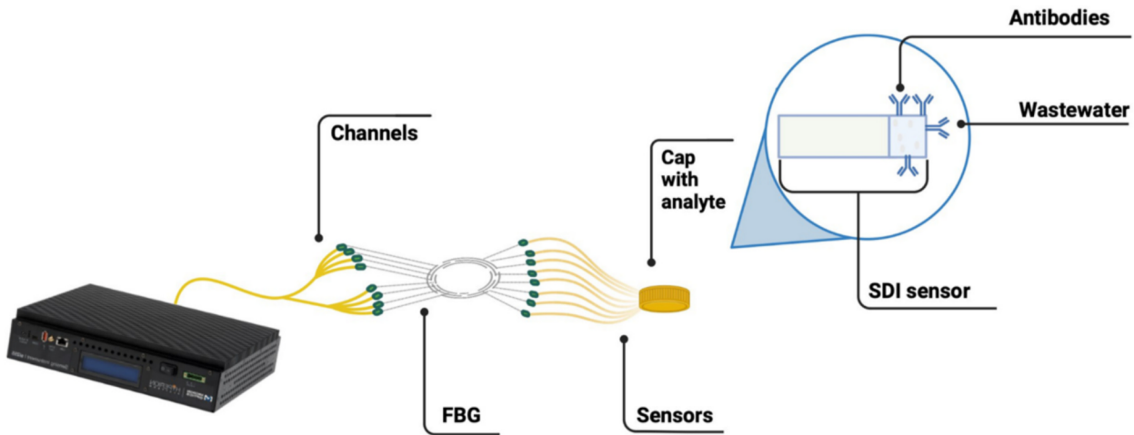
Fig. 3. Setup for measurement of vaccinia virus proteins in wastewater.
