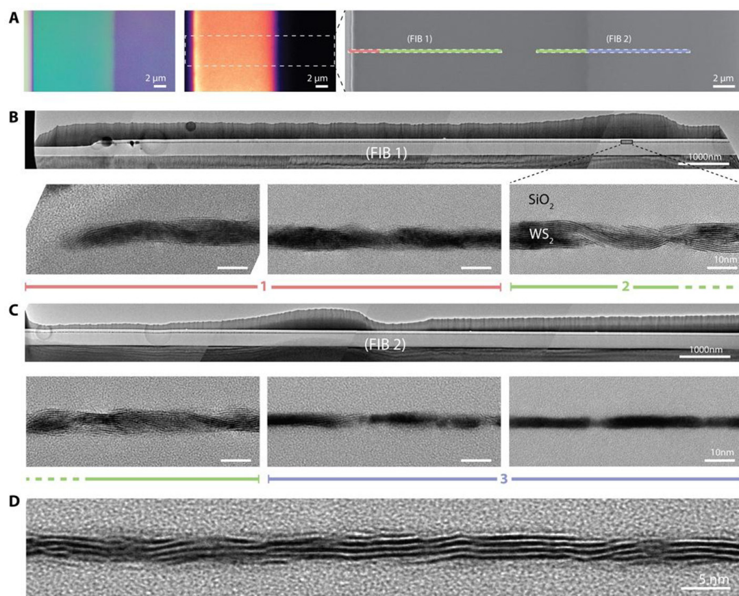
Figure 3. WLRM, Raman, SEM and TEM images of \text{WS}_2 synthesized by lateral conversion. (a) WLRM image (left), Raman map (center), and SEM image showing the regions from which the TEM cross-sectional samples were extracted (right). (b and c) Cross-sectional TEM images showing the \text{WS}_2 layer, sandwiched between \text{SiO}_2 layers, starting from the exposed edge (top left) to the unconverted region (bottom right). The upper images show lower magnification panoramic images of the entire slice, and the lower images show higher magnification images taken from sections approximately above them in the panoramic image. Three regions divided into areas having similar morphological characteristics are labeled 1, 2 and 3. Note that platinum and carbon layers were deposited on top as part of the FIB milling process. (d) Cross-sectional TEM image showing few-layer \text{WS}_2 synthesized by lateral conversion of a 2.4 nm thick \text{WO}_3 film.
