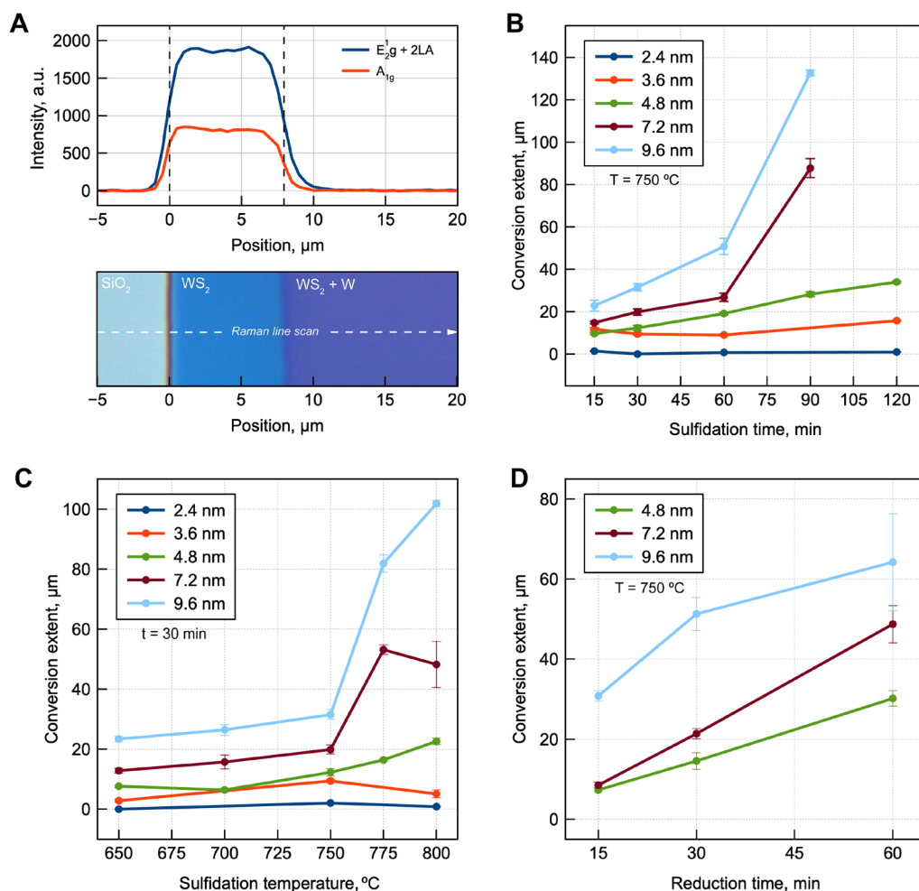
Figure 4. Reaction kinetics of WS 2 lateral conversion. (a) Raman line maps of E_{2g}^1 + 2LA and A_{1g} intensity (top) and optical image (bottom) of the same laterally converted sample, demonstrating that both techniques show similar ELC. (b) Plot showing the extent of conversion as a function of time, holding the temperature constant. (c) Plot showing the extent of conversion as a function of reaction temperature, holding the time constant. (d) Plot showing the extent of conversion as a function of WO x reduction time.
