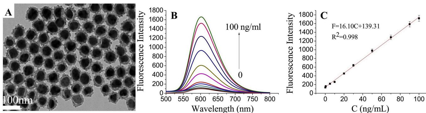
Fig. 6. (A) The TEM micrograph of composite nanoparticles Ag@SiO 2 @SiO 2 -RuBpy of 10 nm SiO 2 spacer thickness; Fluorescence emission spectra of the detection system in the presence of an increasing amount of PSA and calibration curve for PSA detection. (B) Fluorescence emission spectra of the system upon the addition of different concentrations of PSA. (C) Calibration curve for PSA detection. Excitation: 450 nm; Reprinted by the permission of Elsevier, Xu et al. [82].
