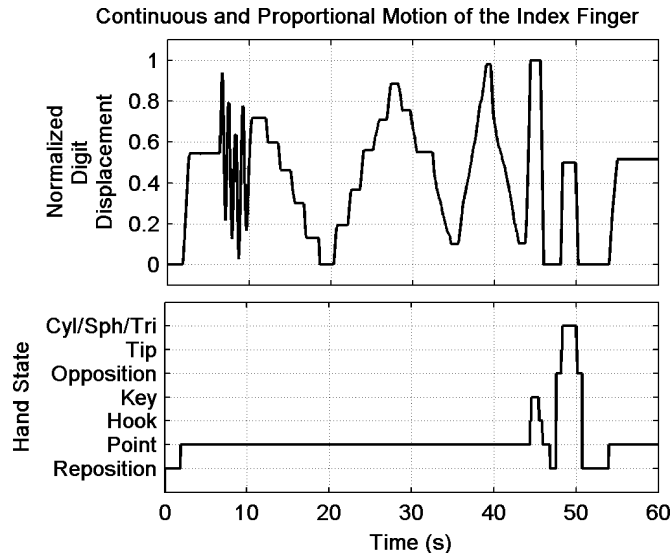
Fig. 7. Plot of normalized digit displacement and hand state during continuous and graded motion of the index finger. High frequency motion, graded motion, low frequency motion, and motion of the index finger during transitions through the state chart are displayed. A video taken during these activities is included in the supplemental materials.
