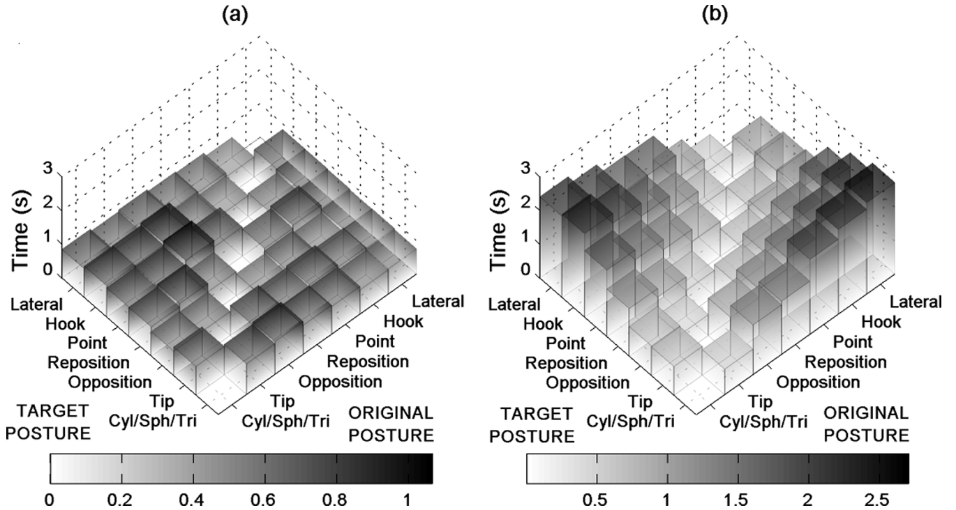
Fig. 5. Average transition times for: (a) the native hand (using the data glove) and (b) multigrasp myoelectric control (using electrodes). Note that the grayscale duration bars are scaled differently for (a) and (b). It can be seen that the transition times are relatively uniform for the native hand while for MMC they are dependent on distance between the original and target posture in the state chart. Note that transition times for adjacent postures with MMC are similar to the average transition time for the native hand.
