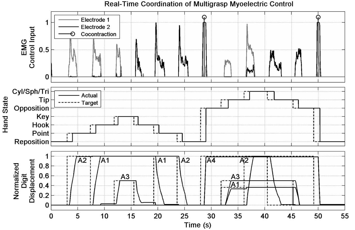
Fig. 6. Plot of EMG Input, Hand State, and Normalized Digit Displacement as a user is prompted through a series of Target Postures. Here, actuator A1 provides digit II flexion and extension, actuator A2 provides coupled flexion and extension of digits III–V, actuator A3 provides digit I flexion and extension, and actuator A4 provides digit I abduction and adduction.
