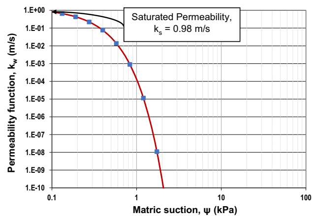
Figure 6. Unsaturated permeability of steel slag.
