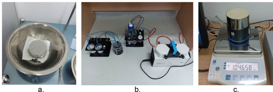
Figure 3. (a) Saturation of the soil specimen, (b) saturation of tensiometers, (c) sensor unit with a soil sample on the balance.
