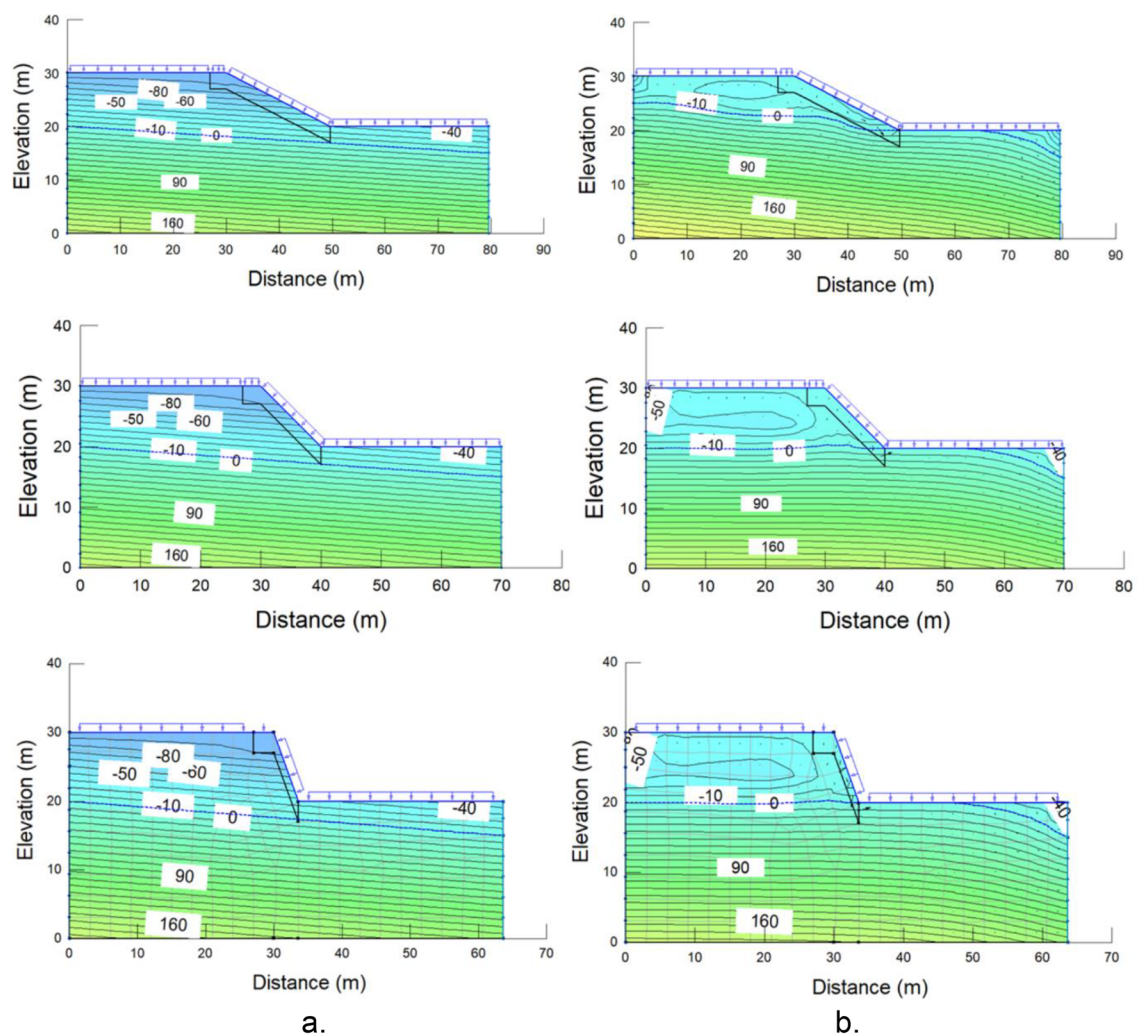
Figure 10. Pore-water pressure contours (a) at t=0 day (before rainfall started) and (b) at t=12 day (at the end of rainfall) for slope height = 10 m and angles = 27° (top); 45° (middle); 70° (bottom).
