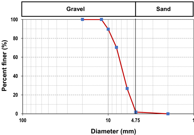
Figure 4. Particle size distribution of steel slag.
