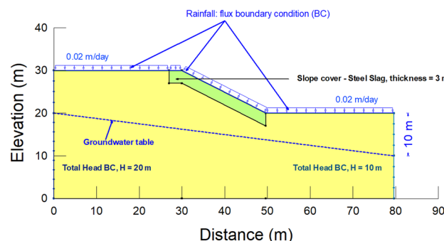
Figure 8. A numerical model for seepage analyses with a slope height of 10 m and slope angle of a 27°
