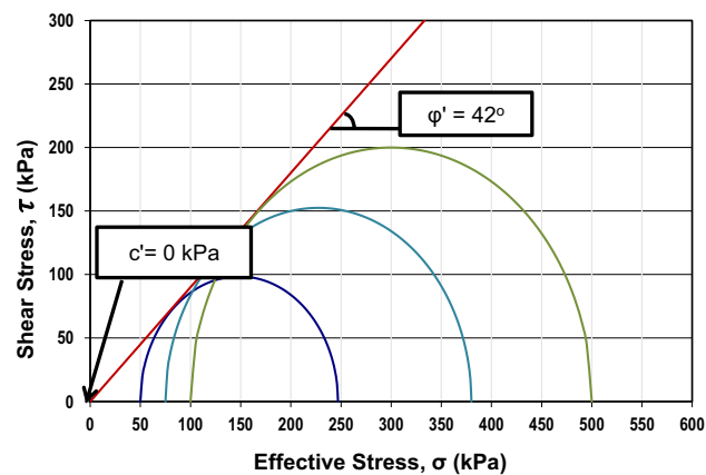
Figure 7. Mohr-Coulomb failure envelope of steel slag constructed from triaxial tests.
