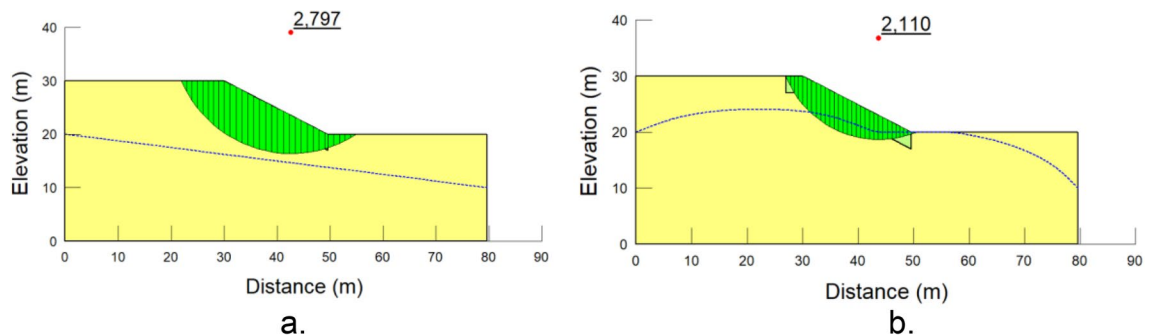
Figure 13. Critical slip surface at (a) t = 0 -day (before rainfall started) and (b) t = 12 day (at the end of rainfall) for slope height = 10 m and slope angle = 27^\circ .
