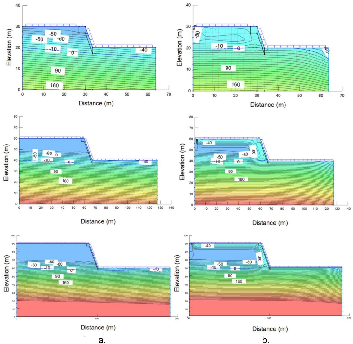
Figure 11. Pore-water pressure contours (a) at t=0 day (before rainfall started) and (b) at t=12 day (at the end of rainfall) for slope angle = 70^\circ and heights = 10 m (top); 20 m (middle); 30 m (bottom).
