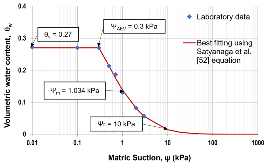
Figure 5. SWCC of steel slag.
