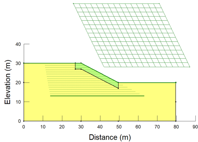
Figure 9. A numerical model for slope stability analyses with a slope height of 10 m and slope angle of a 27°.
