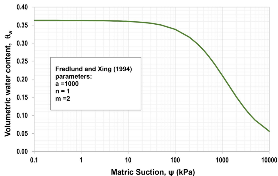
Figure 1. SWCC of the original soil.
