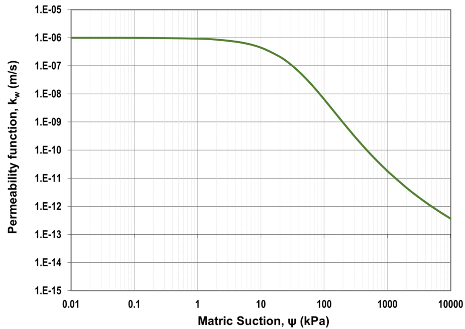
Figure 2. Unsaturated permeability of the original soil.
