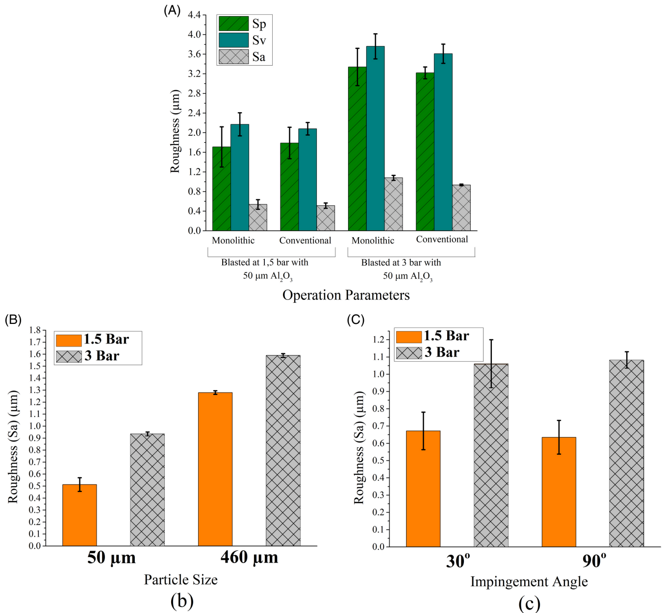
FIGURE 4 Areal surface roughness values of conventional and monolithic zirconia blasted at different parameters: (A) conventional (ICE) and monolithic (CZ) zirconia's at 90°, (B) the effect of particle size on Sa, (C) the effect of impact angles on Sa
