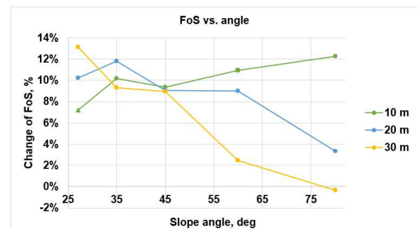
Fig. 6. A factor of safety change at the end of the rainfall against slope angles for three different slope heights.
