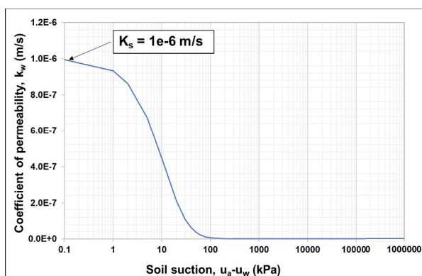
Fig. 2. Permeability function.
