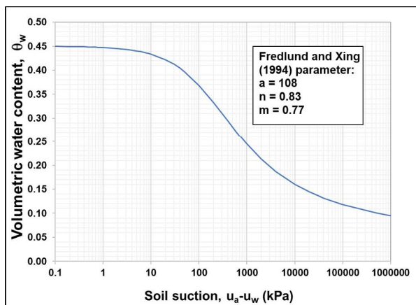
Fig. 1. SWCC curve.
