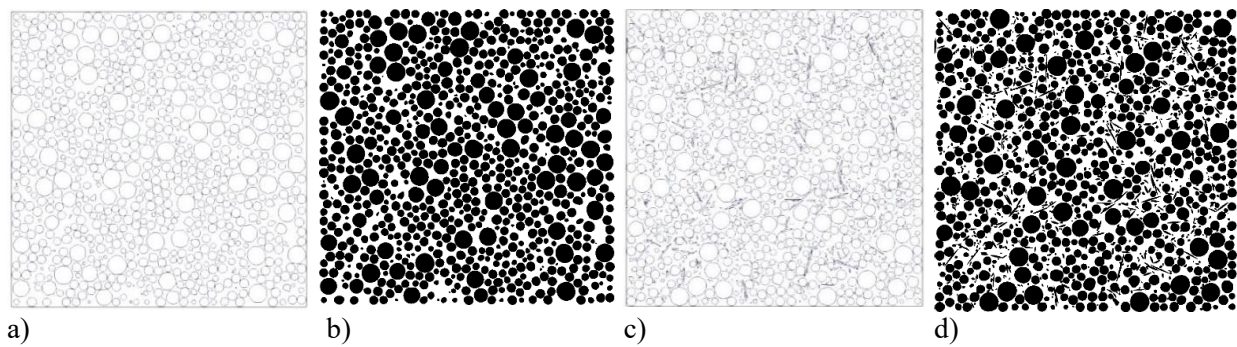
Figure 1. Images of cross-sections normal to Z direction: (a) compact cut from DEM and (b) binary image for Simulation 1, and (c) compact cut from DEM and (d) binary image for Simulation 2.
