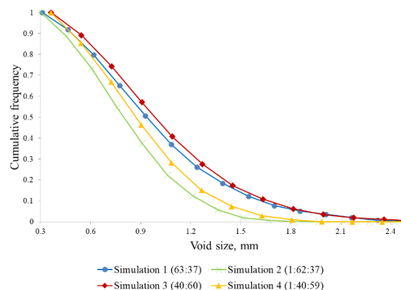
Figure 4. Cumulative frequency void-size distributions measured in Z direction for all samples.
