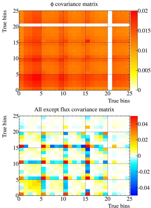
FIG. 11. The fractional covariance matrix obtained from the uncertainties on the flux (top), uncertainties due to all sources except the flux (bottom). The x-axis and y-axis bin numbering is defined in Table XI.
