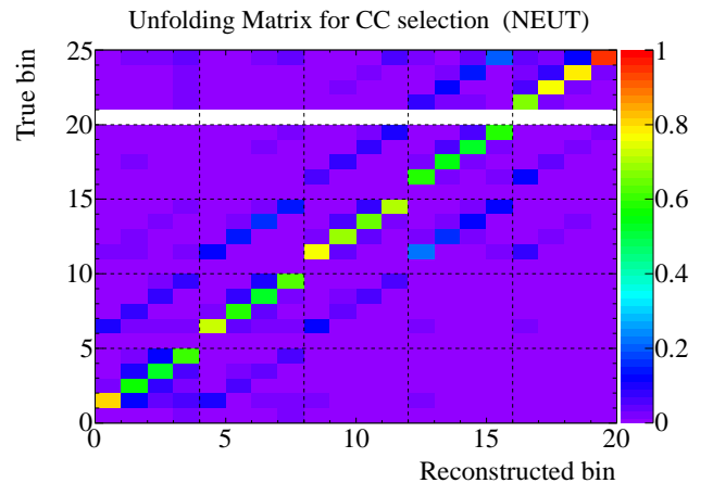
FIG. 10. The unfolding matrix obtained with the NEUT MC simulation. The white line corresponds to backward-going muons in the highest energy bin, for which our MC prediction is zero events. The x-axis and y-axis bin numbering is defined in Table X and Table XI respectively.
