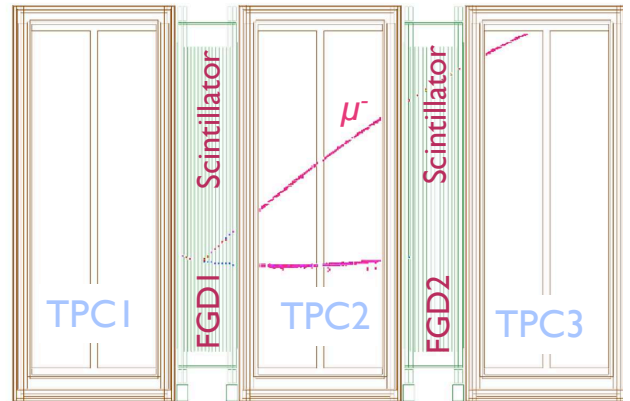
FIG. 5. Side view of a charged current event candidate in the tracker region of the near detector, which shows the bending due to the magnetic field. The muon candidate is reconstructed with an angle of 40^\circ and a momentum of 566 MeV/c.
