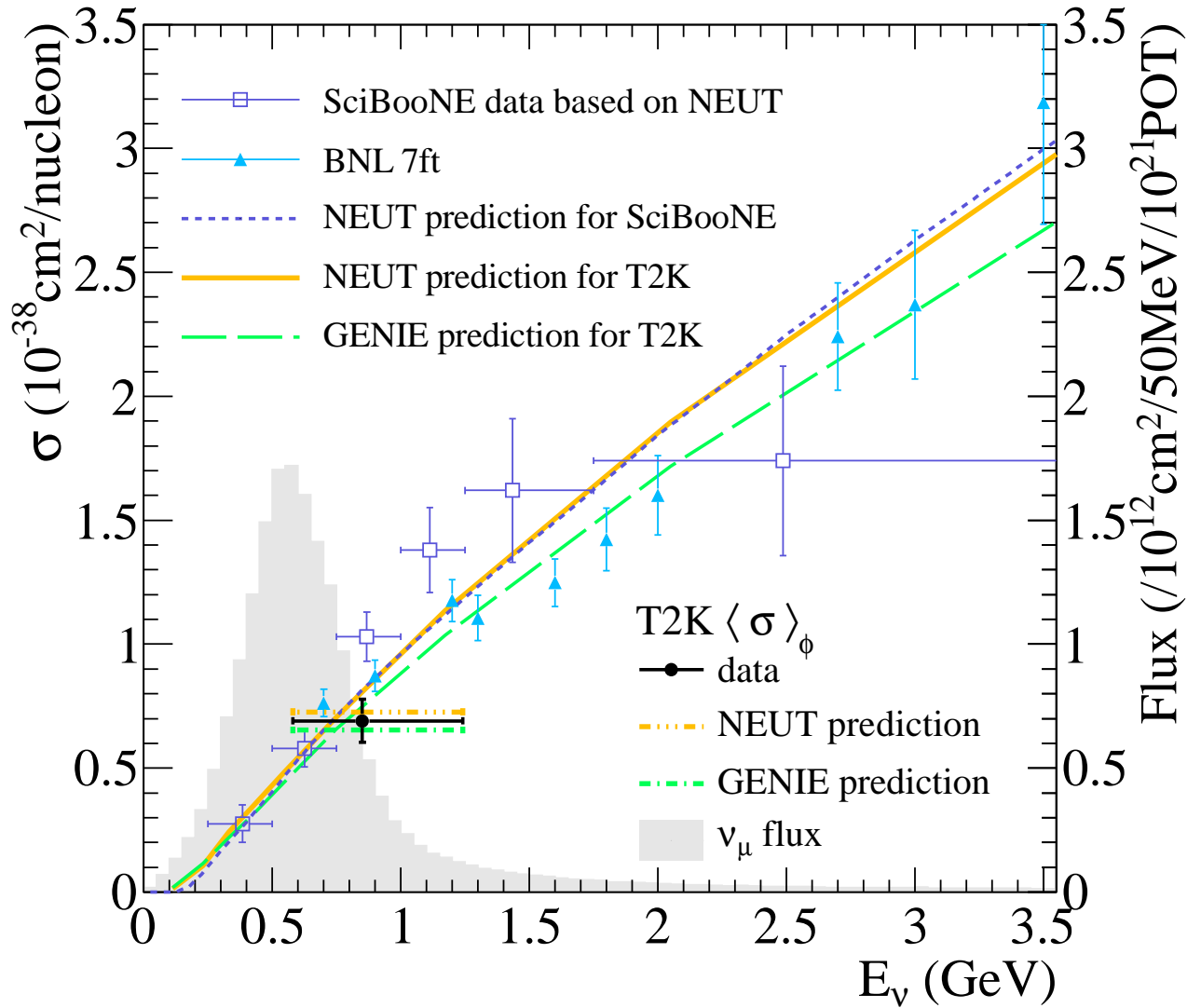
FIG. 13. The T2K total flux-averaged cross section with the NEUT and the GENIE prediction for T2K and SciBooNE. The T2K data point is placed at the flux mean energy. The vertical error represents the total (statistical and systematic) uncertainty, and the horizontal bar represent 68% of the flux at each side of the mean energy. The T2K flux distribution is shown in grey. The predictions for SciBooNE have been done for a C_8H_8 target [51] which is comparable to the mixed T2K target. BNL data has been measured on deuterium [52].
