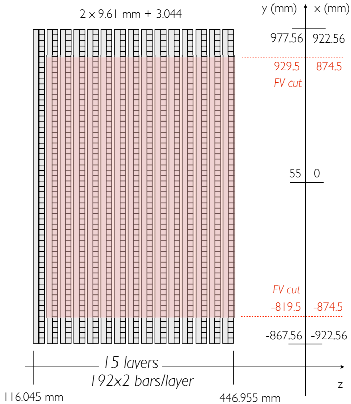
FIG. 4. Schematic view of FGD1 and its fiducial volume (FV) drawn in red. In the y-coordinate, the detector is displaced 55 mm upwards relative to the center of the ND280 coordinate system, which is centered in the magnet.
