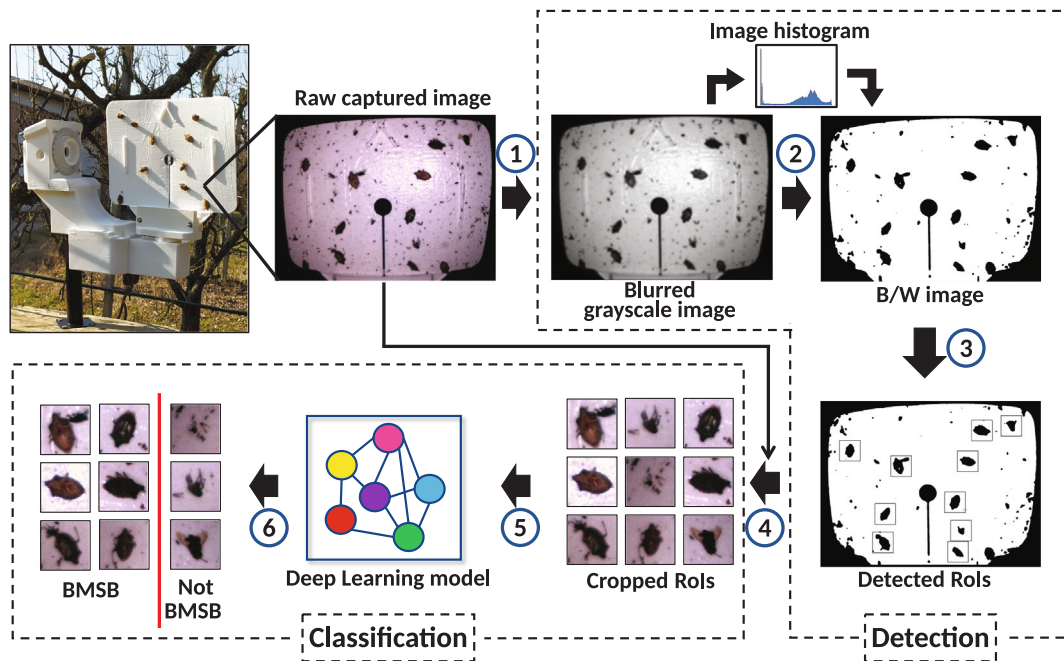
Fig. 4. Image processing algorithm, from the raw captured image to classified Rols.
