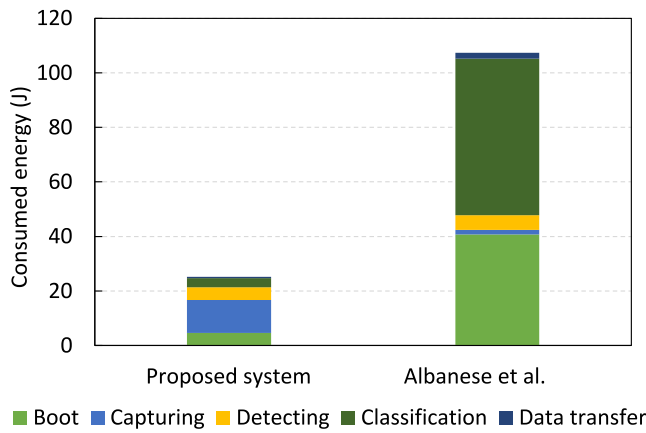
Fig. 10. A breakdown energy consumption of the proposed system and Albanese et al. (2021).
