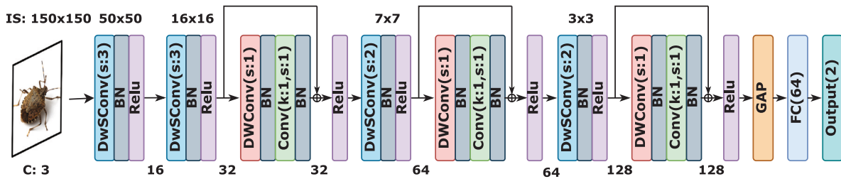
Fig. 6. Proposed classification model; IS: Input Size, C: Number of Channels, DwSConv: Depthwise Separable Convolution, Conv: Convolution, BN: Batch Normalization, GAP: Global Average Pooling, FC: Fully Connected.
