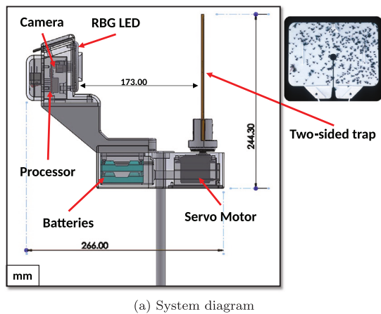
Fig. 2. System overview and components as described in Kargar et al. (2022).
