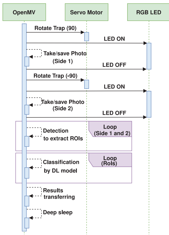
Fig. 3. Diagram of steps followed per cycle.
