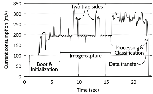
Fig. 9. Proposed system's current consumption over different phases of a cycle.
