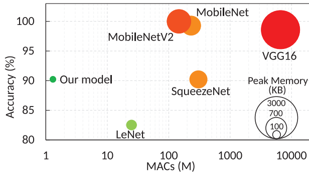
Fig. 8. Comparison of accuracy, complexity (MACs) and peak memory usage; bubbles size represents the peak memory usage, and its colour indicates the possibility of running the corresponding model on typical MCUs.
