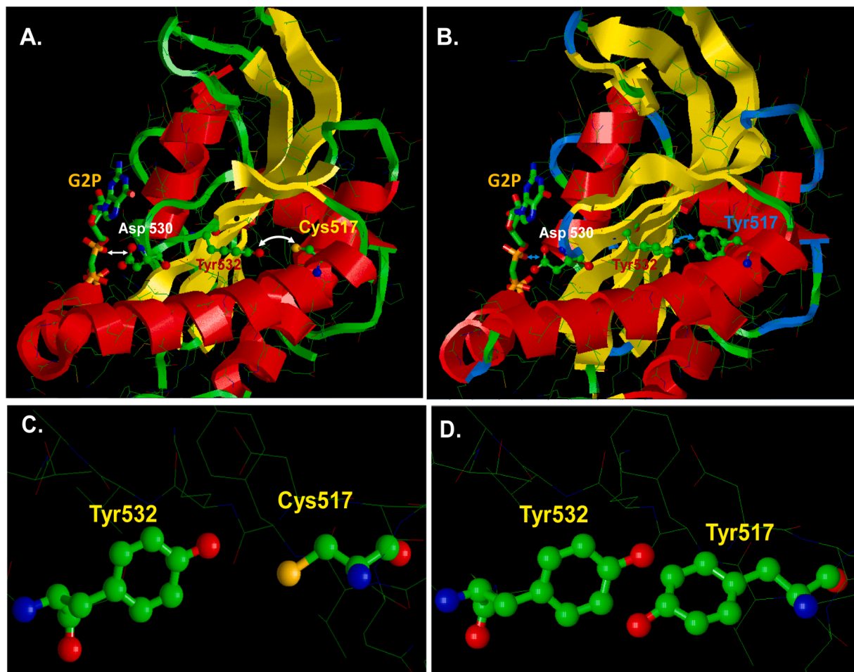
Fig. 7. Molecular modeling of changes in the \alpha_1 sGC catalytic domain induced by Cys517 → Tyr substitution. (A): Close-up view of the \alpha_1 catalytic region of wild type sGC based on the cryo-EM structure of NO-stimulated human sGC (PDB 6JT2). The residues Cys517, Tyr532, Asp530 and the GTP analog are highlighted. (B): Close-up view of the \alpha_1 catalytic region of the \alpha_1 Cys517Tyr \beta_1 mutant. The model was generated using the SWISS-MODEL platform based on PDB 6JT2. The residues Tyr517, Tyr532, Asp530 and the GTP analog G2P (phosphomethylphosphonic acid guanylate ester) are highlighted. For simplicity of viewing, the catalytic region of the \beta_1 subunit is omitted in both (A) and (B). The arrows highlight the cross-talk between residue 517 and Tyr532 and the associated distance between residues Asp530 and the GTP substrate analog. (C-D): Close-up view of residues 517 and Tyr532 shows that in wild type sGC (C) Cys517 and Tyr 532 are more remote than the juxtaposed Tyr517 and Tyr532 in \alpha_1 Cys517Tyr \beta_1 mutant (D).
