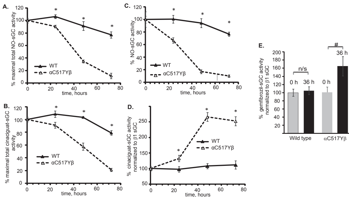
Fig. 6. Time-dependent change in sGC activity in rotenone/antimycin-treated cells. COS-7 cells transiently expressing wild type or \alpha_1 Cys517Tyr \beta_1 sGC were treated with 1 \mu M rotenone and 1 \mu M antimycin. At indicated times, the cells were lysed and sGC activity in response to 10 \mu M DEA-NO (A) or 2 \mu M cinaciguat (B) was measured. Data normalized to total protein lysate are presented as % of cGMP-forming activity in non-treated cells. Data from three independent transfections are presented as mean \pm SD. All activity measurements were performed in triplicates. (C-D): Apparent sGC specific activity calculated after normalization to the amount of \beta_1 sGC determined by western blotting from (A-B). (E): Apparent specific activity of sGC stimulated by 100 \mu M gemfibrozil in control lysates and after 36 h of rotenone/antimycin treatment. Data in (C-E) are presented as % of mean \pm SD of controls. Data from three independent transfections are shown. All measurements were performed in triplicates. * indicates p < 0.05 , two-way ANOVA followed by Bonferroni multi-comparison test; # indicates p < 0.05 vs. control untreated sample ( t -test); n/s – the difference is not statistically significant.
