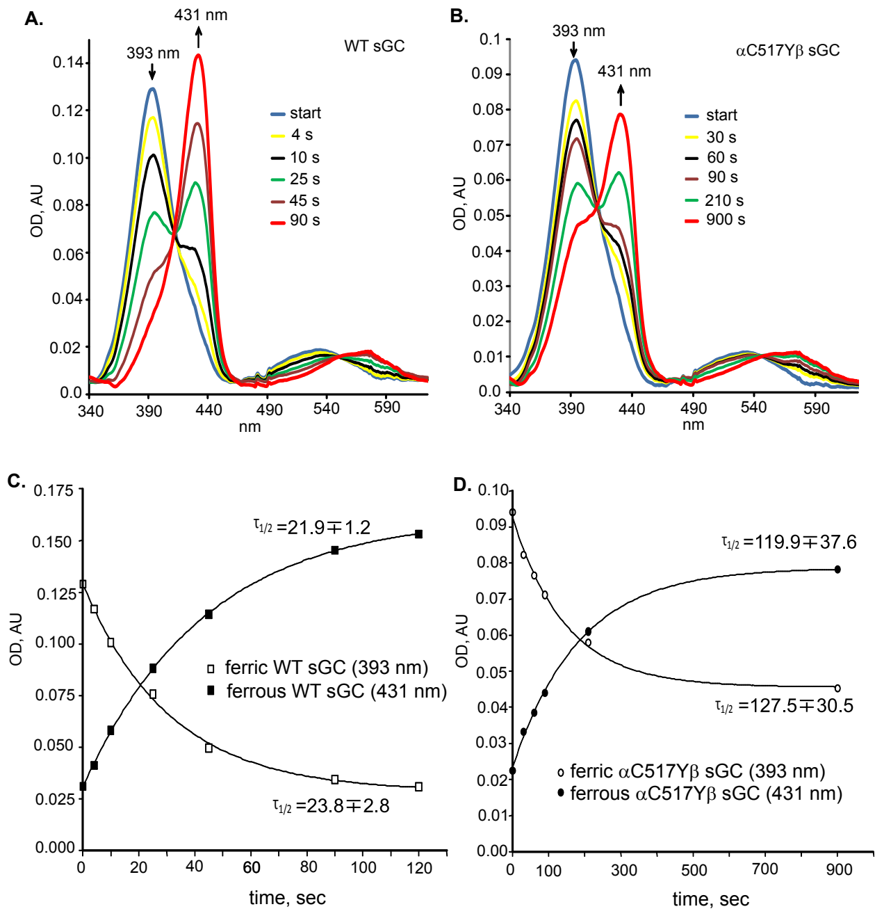
Fig. 4. Kinetics of heme reduction by DTT. Wild type (A) or \alpha_1 Cys517Tyr \beta_1 (B) sGC enzyme preparations containing ferric heme were supplemented with 2 mM DTT and the changes in the UV-Vis spectra were recorded at indicated time points at 25 °C in 50 mM triethanolamine pH 7.4, 250 mM NaCl, 1 mM MgCl 2 . Arrows indicate the position and the direction of absorbance change for ferric and ferrous heme. (C and D): Kinetics of change in the absorbance of ferric (393 nm) and ferrous (430 nm) forms of wild type (C) or \alpha_1 Cys517Tyr \beta_1 (D) sGC heme after the addition of DTT were derived from the data presented in (A) and (B). The calculated half-life of each species is indicated.
