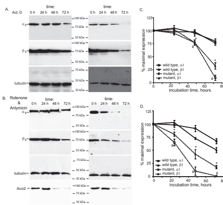
Fig. 5. Diminished stability of \alpha_1 Cys517Tyr \beta_1 sGC in COS7 cells. (A-B): COS-7 cells were transfected with plasmids expressing wild type or \alpha_1 Cys517Tyr \beta_1 sGC. 48 h post-transfection, the cells were treated with 1 \mu M actinomycin D (A) or 1 \mu M rotenone and 1 \mu M antimycin (B). At indicated time points, the cells were lysed and 100,000xg supernatant were used for the detection of \alpha_1 , \beta_1 and \beta -tubulin by western blotting. Changes in the level of ROS sensitive mitochondrial aconitase (ACO2) was evaluated in 20,000xg pellets. Shown are representative blots of three independent transfections with similar results. (C-D): Densitometry results of western blots from (A-B) showing changes in the amount of \alpha_1 and \beta_1 subunits in COS-7 cells expressing wild type or \alpha_1 Cys517Tyr \beta_1 after actinomycin D (A) or rotenone + antimycin (B) treatments. Signals for \alpha_1 and \beta_1 subunits are normalized to \beta -tubulin signal. Data are presented as % of signal obtained in control samples, before the exposure to actinomycin D (A) or rotenone + antimycin (B). Data are mean \pm SD from three independent transfections.
