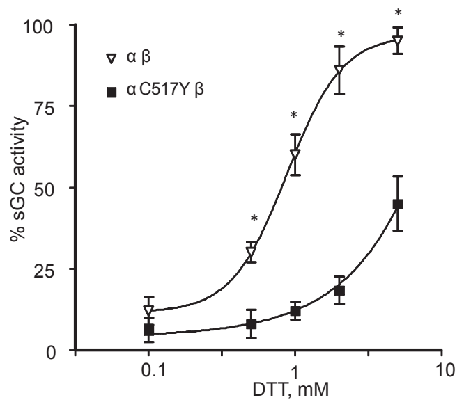
Fig. 3. DTT reactivation of ferric sGC. NO stimulated cGMP forming activity of purified \alpha_1\text{Cys517Tyr}\beta_1 (filled squares) and wild type \alpha_1\beta_1 (open triangles) sGC fully oxidized by 10 \mu\text{M} NS2028 was determined in the presence of indicated concentrations of DTT. Data are presented as % of maximal NO-stimulated activity determined with enzymes preps that were not exposed to NS2028. Data are mean \pm SD from three independent measurements performed in triplicates. * - p < 0.05 (two-way ANOVA followed by Bonferroni multi-comparison test).
