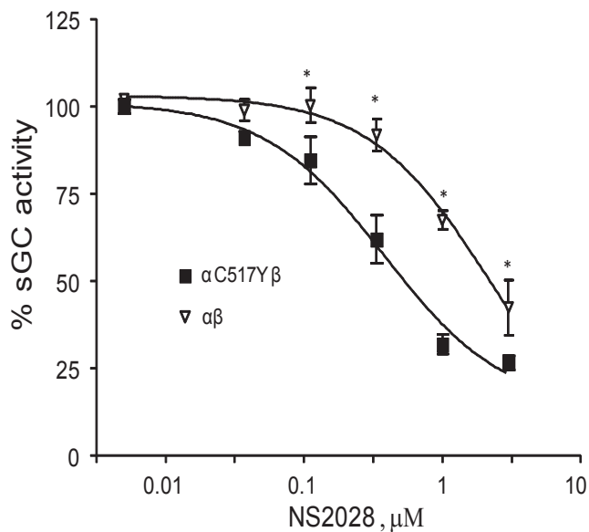
Fig. 2. \alpha_1\text{Cys517Tyr}\beta_1 mutant is more susceptible to heme oxidation. NO stimulated (10 \mu\text{M} DEA-NO) cGMP-forming activity of purified \alpha_1\text{Cys517Tyr}\beta_1 (filled squares) and wild type \alpha_1\beta_1 sGC (open triangles) pre-treated for 5 min with indicated concentrations of heme-oxidizing NS2028 was determined in thiol-free conditions. Data are presented as % of maximal NO-stimulated activity determined in the absence of NS2028. Data are mean \pm SD from three independent measurements performed in triplicates. Maximal activity was 16.02 \pm 0.32 and 3.2 \pm 0.12 \mu\text{mole cGMP}/\text{min}/\text{mg} for wild type and mutant sGC, respectively. EC50 for NS2028 was estimated at 2.18 \pm 0.15 \mu\text{M} for wild type sGC and 0.37 \pm 0.13 \mu\text{M} for the mutant sGC. * - p < 0.05 (two-way ANOVA followed by Bonferroni multi-comparison test).
