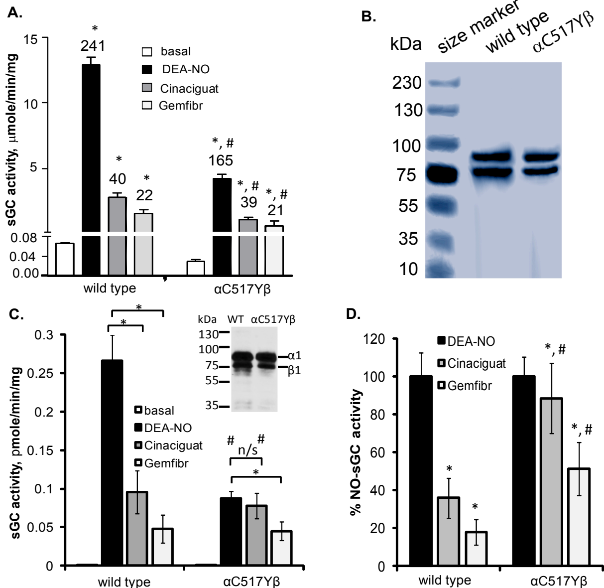
Fig. 1. Comparison of NO, cinaciguat and gemfibrozil response of purified wild type and \alpha_1 Cys517Tyr \beta_1 and in COS7 cells. (A): Specific activity of purified wild type and \alpha_1 Cys517Tyr \beta_1 in basal conditions and after stimulation with 10 \mu M DEA-NO, 1 \mu M Cinaciguat or 100 \mu M Gemfibrozil (Gemfibr). Numbers above bars indicate the fold stimulation over basal activity. The assay was performed with 1 mM DTT. Data are mean \pm SD from three independent experiments performed in triplicate. * indicates p < 0.05 vs basal activity ( t -test); # indicates p < 0.05 vs. wild type values (one-way ANOVA followed by Tukey's multi comparison test). (B) Coomassie staining of wild type and \alpha_1 Cys517Tyr \beta_1 enzyme preparations. 5 \mu g purified protein was displayed on SDS-PAGE and stained with Coomassie blue dye. (C): cGMP-forming activity of COS7 cells transfected with plasmids expressing wild type sGC or the rare \alpha_1 Cys517Tyr \beta_1 variant. The activity was measured in the presence of 10 \mu M DEA-NO, 1 \mu M Cinaciguat or 100 \mu M Gemfibrozil, without DTT. Data are mean \pm SD from measurements performed in triplicates from three independent transfections. * indicates p < 0.05 (indicated t -test); # indicates p < 0.05 vs. wild type values (one-way ANOVA followed by Tukey's multi comparison test). n/s- difference not statistically significant. Inset: expression of \alpha_1 and \beta_1 subunits in 100 \mu g of COS-7 cell protein lysate transfected by wild type or \alpha_1 Cys517Tyr \beta_1 sGC. (D): cGMP-forming activity data from (C) presented as percent of NO-stimulated activity. * indicates p < 0.05 vs NO-stimulated activity ( t -test); # indicates p < 0.05 vs. wild type values (one-way ANOVA followed by Tukey's multi comparison test). (For interpretation of the references to colour in this figure legend, the reader is referred to the web version of this article.)
