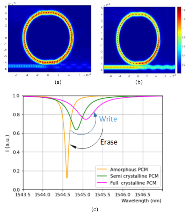
FIGURE 5. (a-b) Finite element Mode simulation of MRR with coupled PCM in (a) amorphous and (b) crystalline states. (c) The change in transmission for an individual memory cell showing Write/Erasing cycling, corresponding to amorphous and crystalline states of the PCM.
