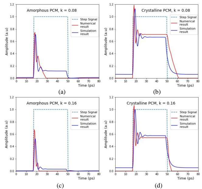
FIGURE 10. Transfer model response with 33 ps step signal. The figures include PCM readings at amorphous and crystalline phase at coupling coefficient ( k ) of 0.08 (a,b) and 0.16(c,d).
