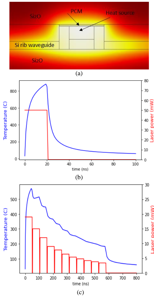
FIGURE 8. (a) PCM waveguide cross section model for Comsol simulation . (b) Amorphous and (c) crystalline heating results from Comsol Multiphysics.
