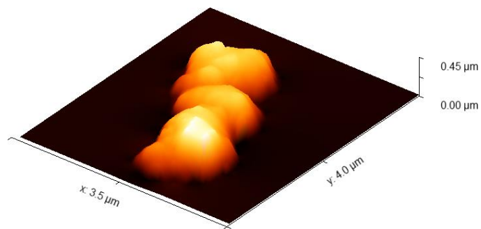
SN_CNPs(200ug/ml)
