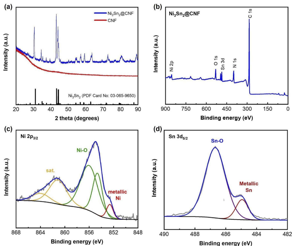
Fig. 1 XRD patterns of both \text{Ni}_3\text{Sn}_2@\text{CNF} and CNF samples (a), XPS survey spectrum (b), Ni 2p_{3/2} (c) and Sn 3d_{5/2} (d) XPS spectra of the \text{Ni}_3\text{Sn}_2@\text{CNF} .
