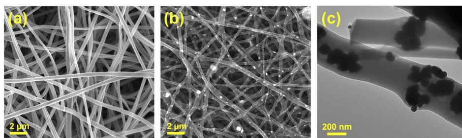
Fig. 2 SEM image of the CNF (a), SEM image (b) and TEM image (c) of the \text{Ni}_3\text{Sn}_2@\text{CNF} .
