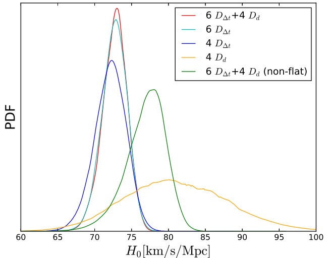
FIG. 1.— The joint posteriors on H_0 are shown for the full data set “6 D_{\Delta t} + 4 D_d ”, the time-delay distances “6 D_{\Delta t} ” and angular distances “4 D_d ” separately, and the change from the previous “4 D_{\Delta t} ” of Liao et al. (2019). Here we assume flatness to compute D_{\Delta t} from the SNe GP by default. For completeness, we also consider the non-flat case for the full data set.
