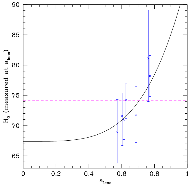
FIG. 6.— Data points show the measured trend in derived Hubble constant H_0 measured from lenses at scale factor a_{\text{lens}} , while the curve is the modified gravity toy model, Eq. (14), for measurements involving light deflection (which for a_{\text{lens}} \ll 1 goes to the true expansion rate H_0 ). The horizontal dashed magenta line shows the value of H_0 quoted by Millon et al. (2019) for the data.
