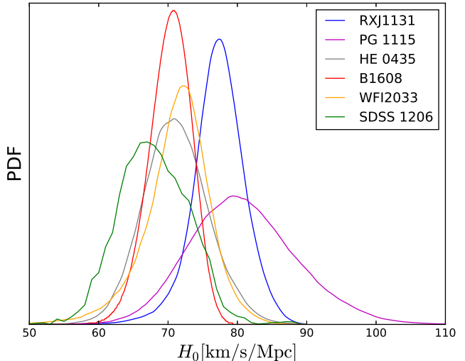
FIG. 2.— The individual posteriors on H_0 from each lensing system are shown, for flat cosmology.
