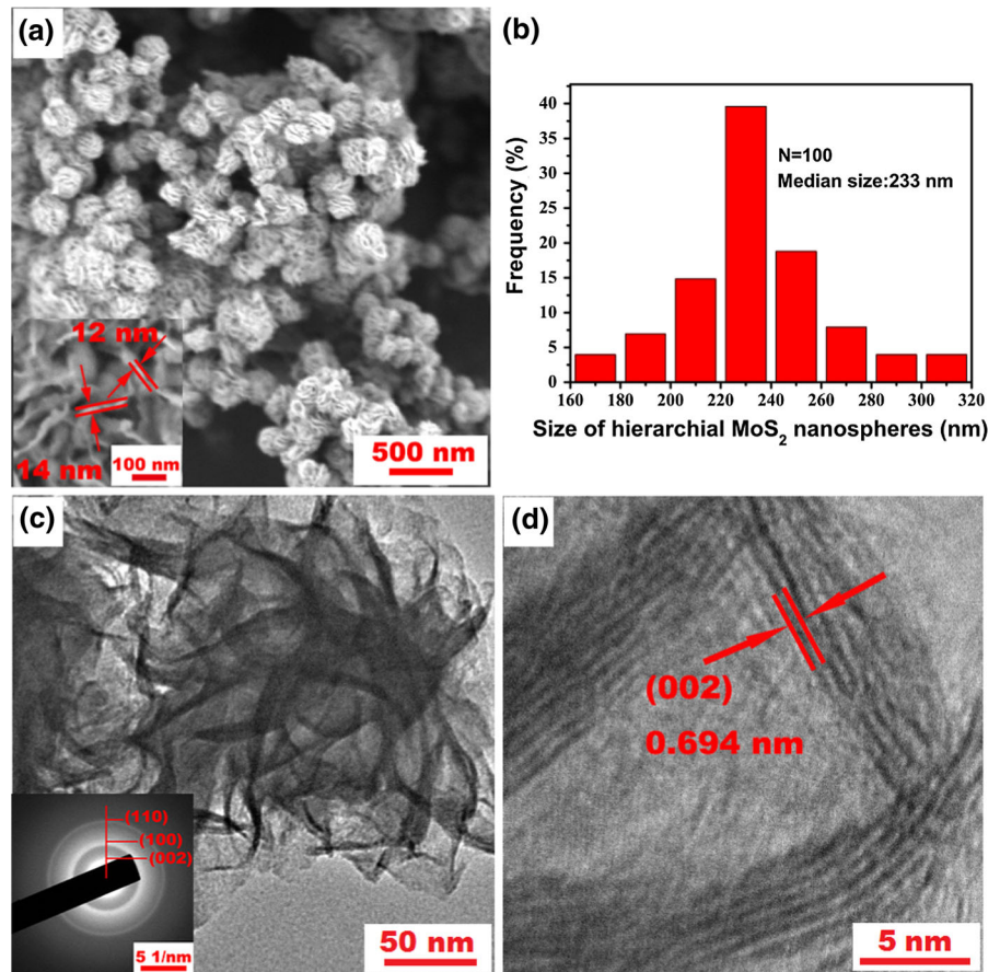
Fig. 3 a Low magnification SEM of the hierarchical MoS 2 microspheres; inset high magnification SEM of the hierarchical MoS 2 microspheres; b particle size distribution of the hierarchical MoS 2 microspheres; c TEM of the hierarchical MoS 2 microspheres, inset SAED pattern of the hierarchical MoS 2 microspheres; d HRTEM of the hierarchical MoS 2 microspheres
