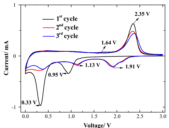
Fig. 4 CV profiles of the hierarchical MoS 2 microsphere anode
