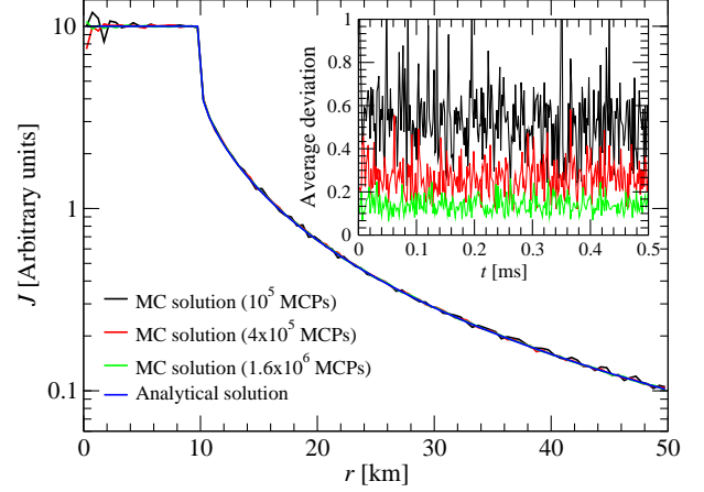
FIG. 3.— The zeroth moment for radiation J as a function of radial coordinate r in the homogeneous sphere test for three simulations in which 10^5 , 4 \times 10^5 , and 1.6 \times 10^6 new MCPs are emitted in each timestep (black, red, and green lines, respectively). Also shown (blue line) is the zeroth moment from the analytical solution. The inset plot shows the average deviation of the zeroth moment in these three Monte Carlo simulations from the analytical solution.
