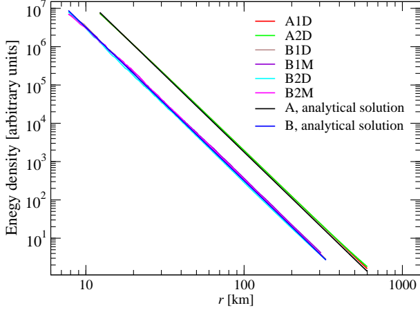
FIG. 13.— The radiation energy density in the comoving frame as a function of the radial coordinate inside homogeneously expanding shell scattering of radiation.
