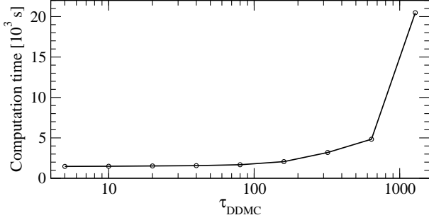
FIG. 10.— Time spent for performing first 500 timesteps as a function of parameter \tau_{\text{DDMC}} for PNS evolution simulations. Since at high optical depth the pure Monte Carlo calculations are more expensive than the DDMC calculations, the computational time increases with \tau_{\text{DDMC}} . Beyond \tau_{\text{DDMC}} > 1280 , our simulations become computationally too expensive, and we do not consider even larger values of \tau_{\text{DDMC}} .
