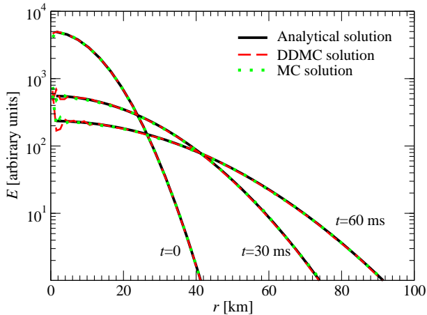
FIG. 4.— The radial profile of the energy density of a Gaussian radiation packet diffusing into a uniform medium with a constant scattering opacity at three different times. The black line corresponds to the analytical solution, the dashed red line is obtained using the DDMC scheme, while the dotted green line is produced by the MC scheme. Note that the fluctuations in the energy density that are particularly visible near the central region at t = 30 ms and t = 60 ms are simply caused by the random noise intrinsic to Monte Carlo methods. This noise is particularly pronounced in central zones because those zones have smaller volumes and thus contain smaller numbers of MCPs. One can reduce this noise by choosing smaller weights for MCPs in central regions. In our test, we use constant weight everywhere for the entire radiation packet. Moreover, these fluctuation decrease with increasing number of MCPs, according to the central limit theorem.
