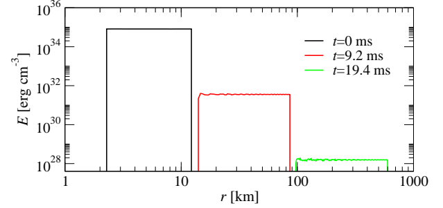
FIG. 12.— The radial profile of the radiation energy density measured by a comoving observer at different times in the homogeneously expanding shell test for simulation A1D using 1,280,000 MC particles. See the discussion in the main text for further details of the simulation.
