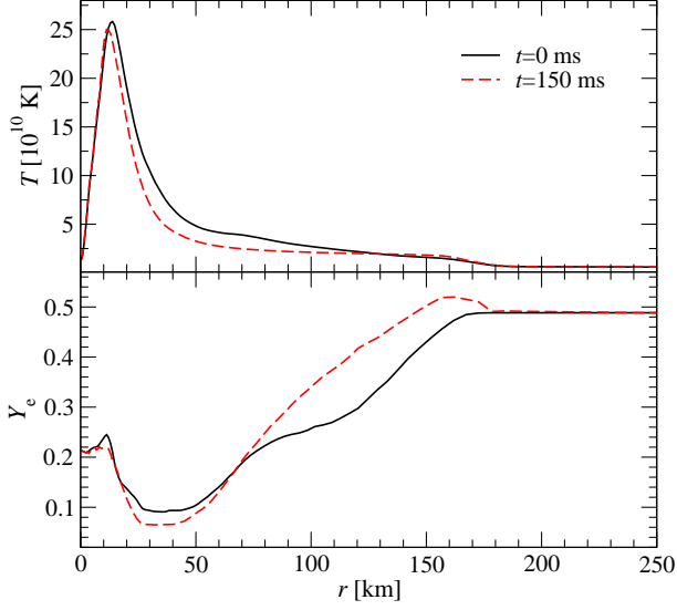
FIG. 9.— The radial profiles of the temperature T and electron fraction Y_e at t = 0 and t = 150 ms after the start of simulation.
