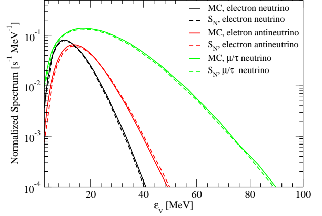
FIG. 6.— The stationary state neutrino spectra at 300 km normalized by the total luminosity obtained with our Monte Carlo scheme (solid lines). For comparison, we show results obtained by Ott et al. (2008) with an S_N code (dashed lines).
