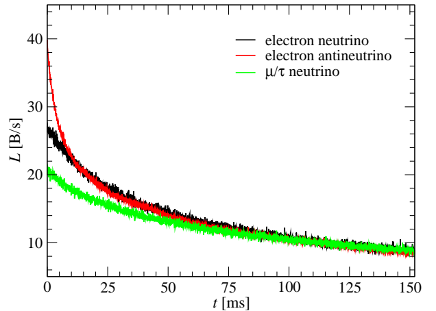
FIG. 8.— Luminosity as a function of time in our PNS evolution calculation.
