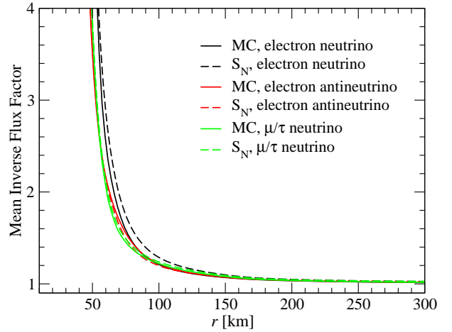
FIG. 7.— The stationary state radial profiles of the mean inverse flux factors for the three different types of neutrinos obtained with our Monte Carlo scheme (solid lines). For comparison, we show results obtained by Ott et al. (2008) with an S_N code (dashed lines).
