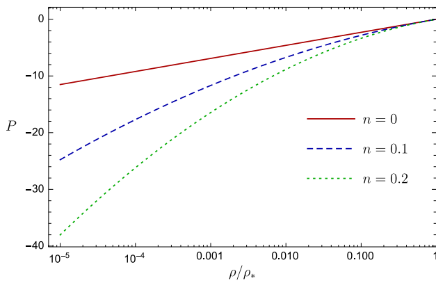
Fig. 1 Pressure as a function of the density in extended logotropic models (cf. Eq. (5)). The different curves correspond to different values of the parameter n , while we have assumed A = 1
