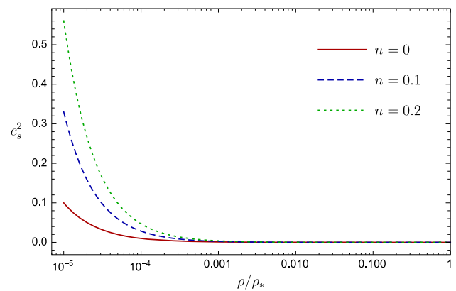
Fig. 3 Quadratic speed of speed as a function of the density in extended logotropic models (cf. Eq. (7)). The different curves correspond to different values of the parameter n , while we have assumed A/\rho_* = 10^{-6}
