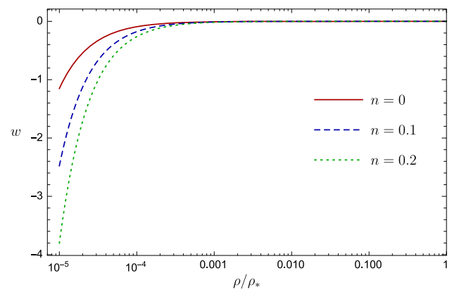
Fig. 2 Equation of state parameter as a function of the density in extended logotropic models (cf. Eq. (6)). The different curves correspond to different values of the parameter n , while we have assumed A/\rho_* = 10^{-6}
