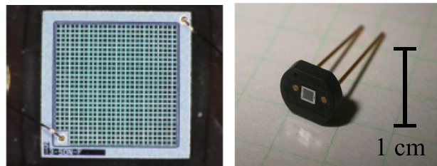
Figure 10: Photographs of an MPPC with a sensitive area of 1.3 \times 1.3 \text{ mm}^2 : magnified face view (left) with 667 pixels in a 26 \times 26 array (a 9-pixel square in the corner is occupied by an electrode); the ceramic package of this MPPC (right).
