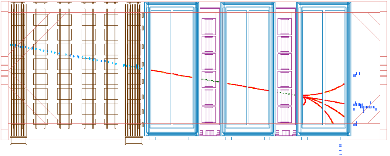
Figure 28: This event display shows an event with a muon track entering via the front face of the \text{P}\text{O}\text{D} detector, continuing to the tracker (TPC and FGD) region and producing secondary particles on the way. The secondary particles are then stopped in the ECal detectors.
