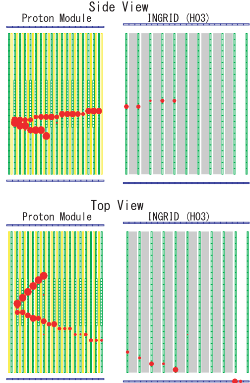
Figure 15: A typical neutrino event in the Proton Module. A neutrino enters from the left and interacts within the module, producing charged particles whose tracks are shown as the red circles. One of them exits the Proton Module and enters the central INGRID horizontal module. Each of the green cells in this figure is a scintillator, and the size of the red circles indicates the size of the observed signal in that cell. Blue cells indicate veto scintillators.
