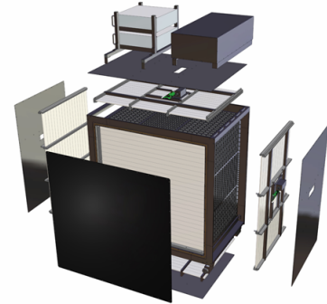
Figure 13: The Proton Module. Similar to the INGRID modules, but with finer grain scintillator and without the iron plates.
